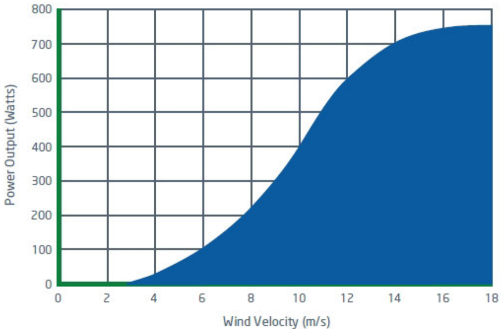
LE-600 Power curve
